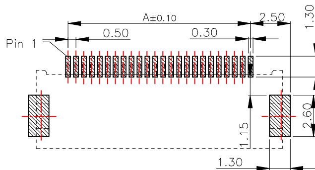
RECOMMEND PCB LAYOUT
