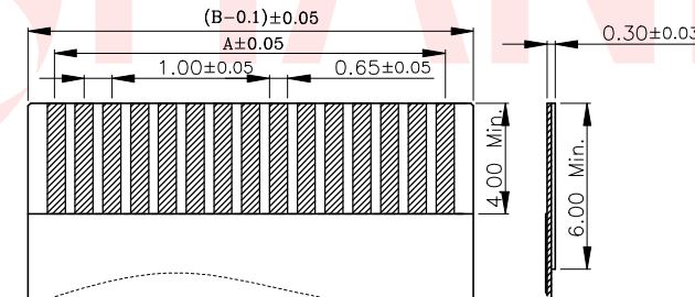
适用扁平线 (Applicable Flat Cable)
