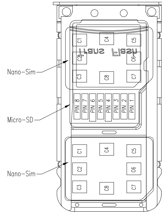
BOTTOM VIEW
