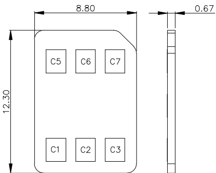
SIM CARD LAYOUT
