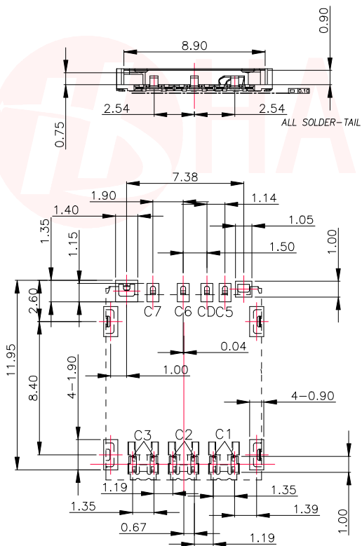
RECOMMENDED PCB LAYOUT TOP VIEW (TOLERANCE: ±0.05) RECOMMENDED METAL MASK T=0.12MM
