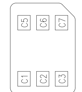
NANO SIM CARD PAD
