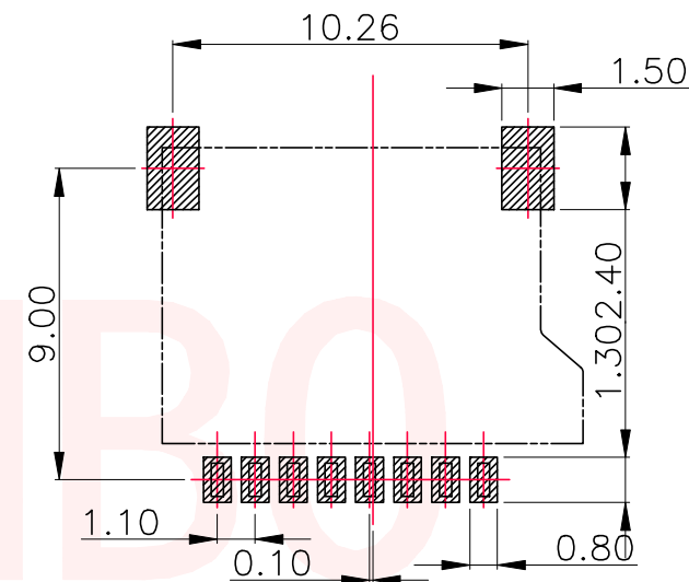
RECOMMENDED PCB LAYOUT (Witchout Post)
