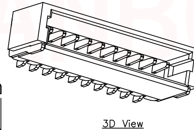
3D View
