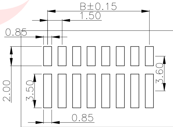
PCB Layout
