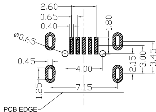
RECOMMENDED PCB LAYOUT TOLERANCE: \pm 0.05
