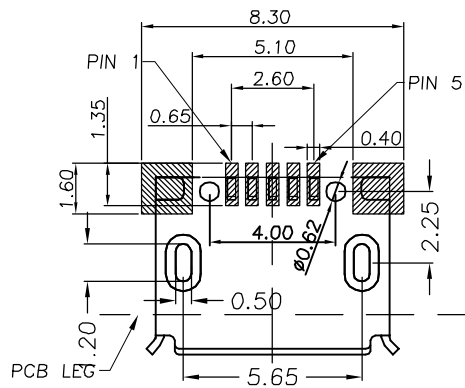
RECOMMENDED P.C.B. LAYOUT TOP VIEW (TOLRANCE: ±0.05)
