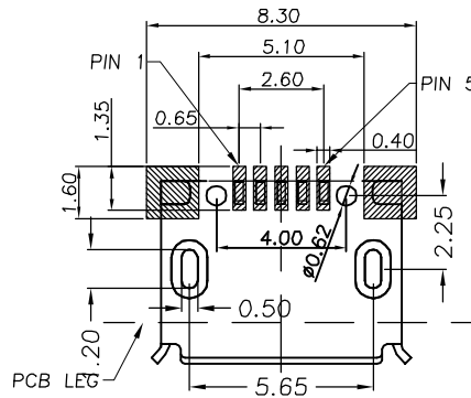
RECOMMENDED P.C.B. LAYOUT TOP VIEW (TOLRANCE: ±0.05)
