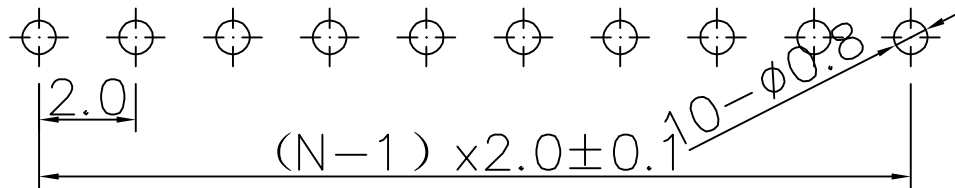
P. C. B Layout
