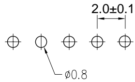
Recommended P.C. Board Hole Layout
