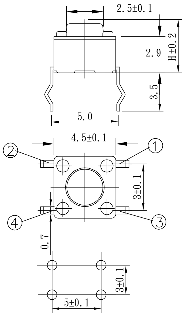
Printed circuit board mounting hole dimension
