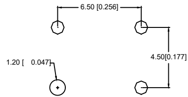
PCB.WELDING DRAWING
