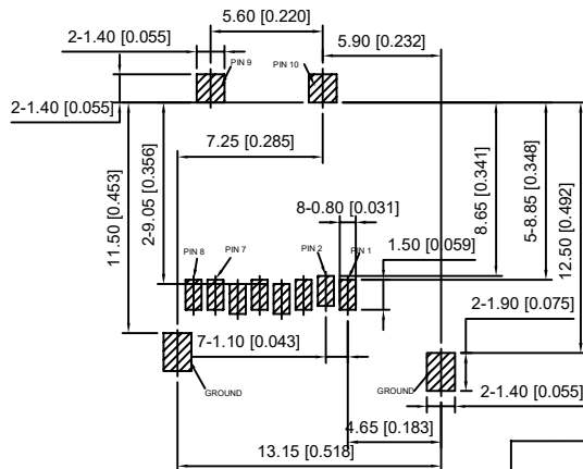
RECOMMENDED PCB LAYOUT (ALL TOLERANCE ARE ±0.05)
