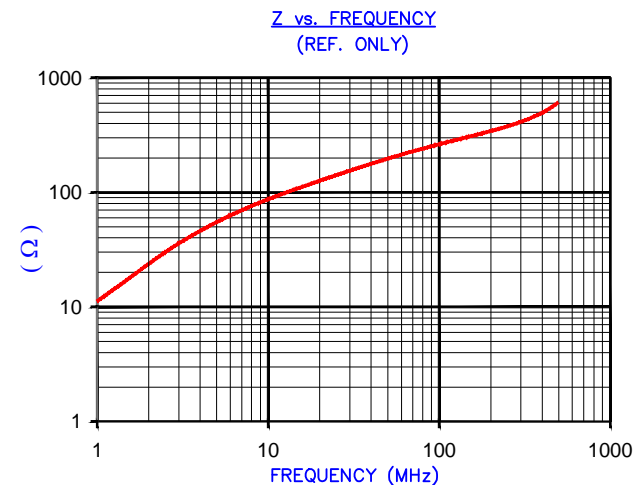
AGILENT E4991A Impedance/Material Analyzer HP 16194A
