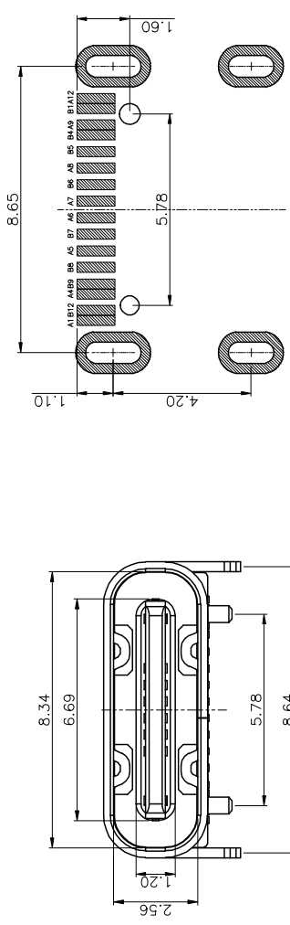
PCB LAYOUT(Recommend) (General Tolerance:±0.05)
