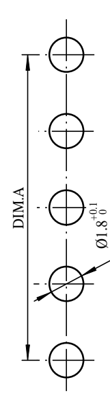
PCB LAYOUT
