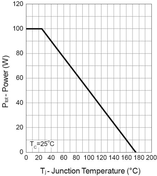
Power Dissipation
