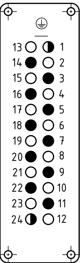
contact arrangement (view from termination side)
