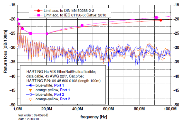
Return loss:
