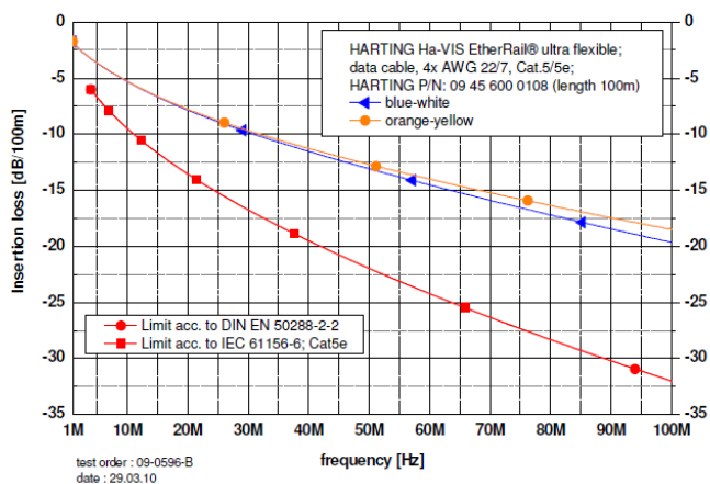
Attenuation:
