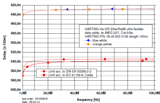
Propagation Delay:
