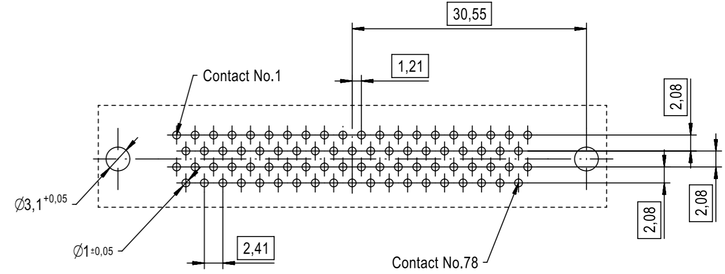
PC-Board layout view component side thickness 1,6 mm
