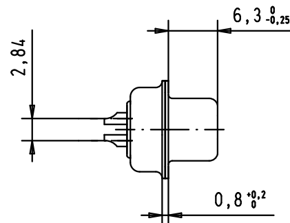
Solder bucket for AWG 20
