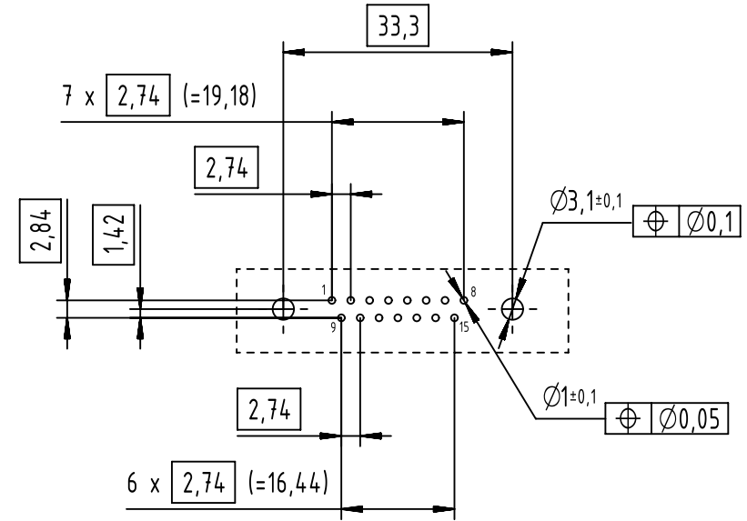
Connector retention and insertion forces on PC-Board: 25 N / 80 N
