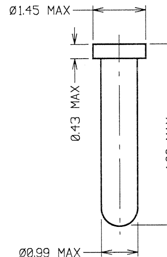
DETAILED VIEW OF SOCKET H3191-XX
