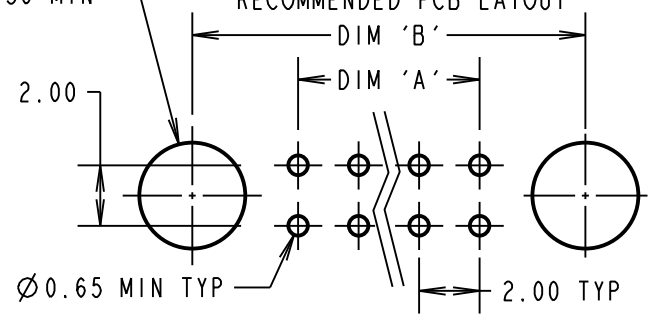
SECTION X-X RECOMMENDED PCB LAYOUT
