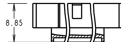
1mm POTTING WALL (M80-576XX05A)
