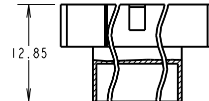
5mm POTTING WALL (M80-576XX05)
