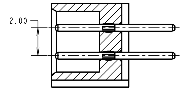
SECTION X-X
