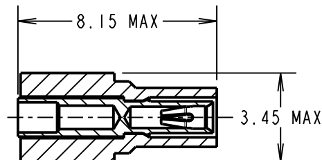
SECTION X-X
