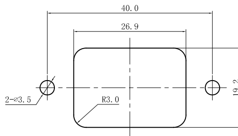
PANEL CUT-OUT
