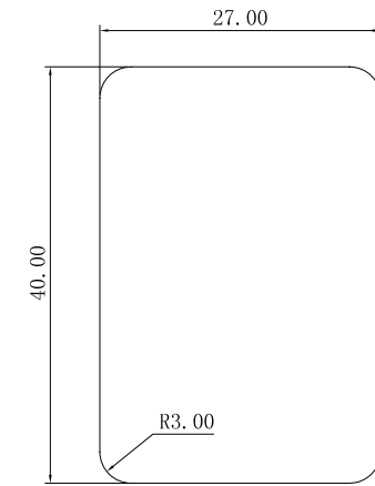
PANEL CUT-OUT
