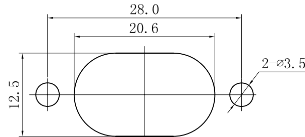
PANEL CUT-OUT
