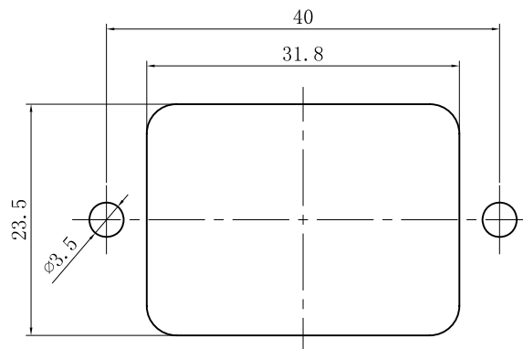
PANEL CUT-OUT
