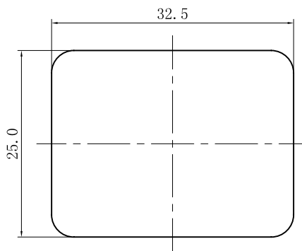
PANEL CUT-OUT
