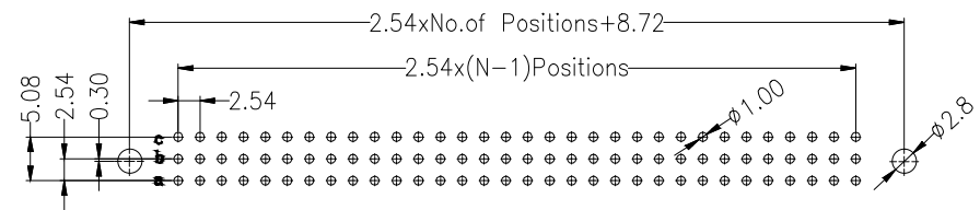
Recommended P.C.B Layout(Top Side) (PCB BOARD TOLERANCE±0.05)
