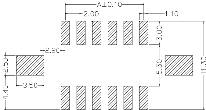
PCB LAYOUT
