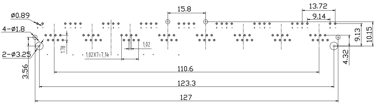
PC Board Layout Component Side Shown
