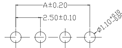
PCB LAYOUT
