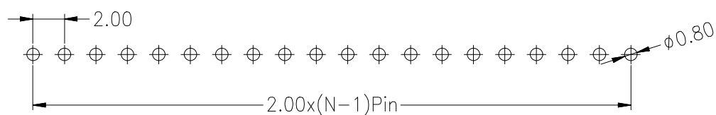
Recommended P.C.B Layout(Top Side) (PCB BOARD TOLERANCE \pm 0.05 )
