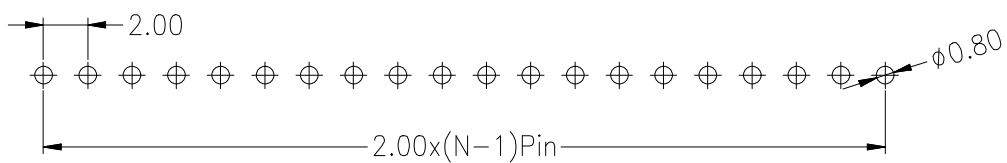
Recommended P.C.B Layout(Top Side) (PCB BOARD TOLERANCE±0.05)
