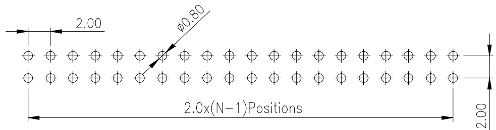
Recommended P.C.B Layout(Top Side) (PCB BOARD TOLERANCE±0.05)
