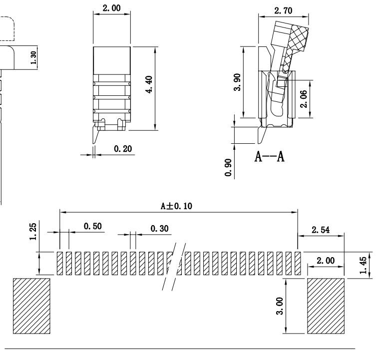
PCB Layout
