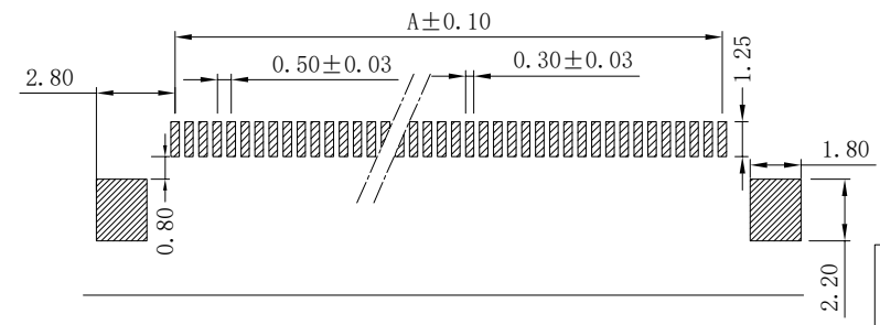
PCB Layout
