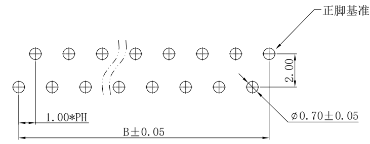
PCB LAYOUT
