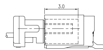
MATED CONDITION
