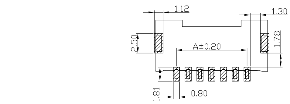
P.C.B LAYOUT TOLERANCE: ±0.05
