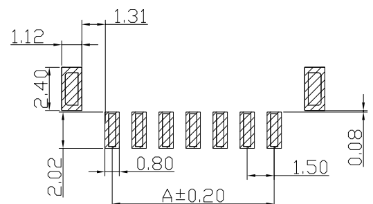
P. C. B LAYOUT TOLERANCE: ±0.05
