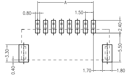
PCB LAYOUT(Tolerance:±0.05)
