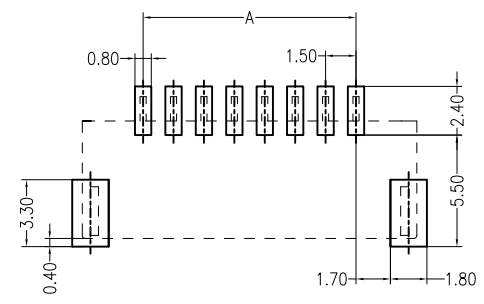
PCB LAYOUT(Tolerance:±0.05)
